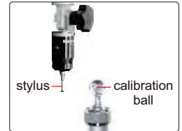
stylus — calibration ball probe ( optional ), includes Ø2mm and Ø3mm styli, Ø25mm calibration ball, measuring accuracy is 10µm
